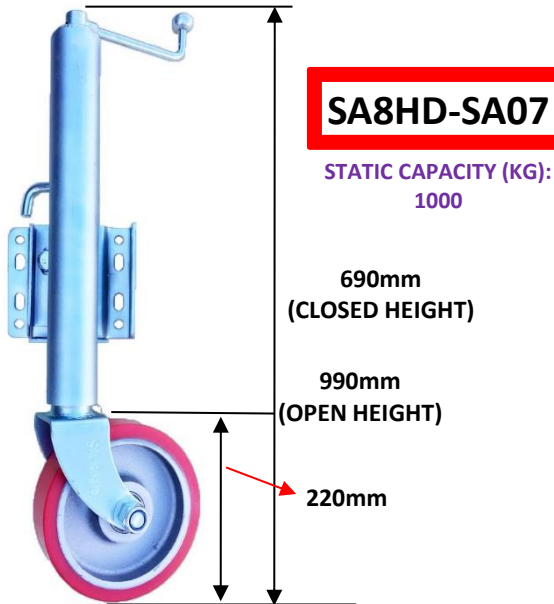
8 x 2 HEAVY DUTY JOCKEY WHEEL c/w SINGLE LOCKING PIN BRACKET
