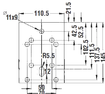
Boltdown Specs.
