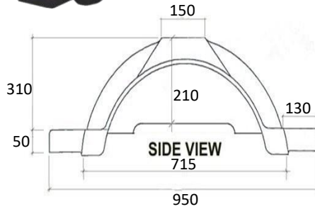
13" PLASTIC MUDGUARDS
