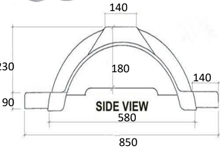
10" PLASTIC MUDGUARDS
